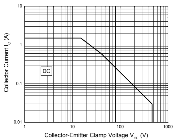
Figure 4. Safe Operating Areas (TO-126 Package)
