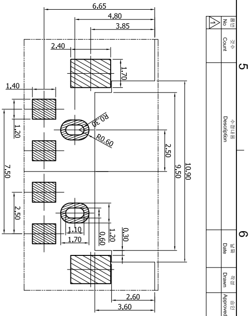
PCB Layout Recommend Tolerance = ±0.05
