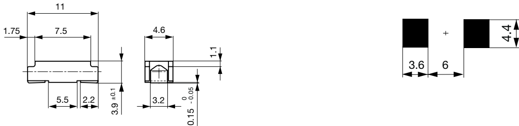
Soldering pads
