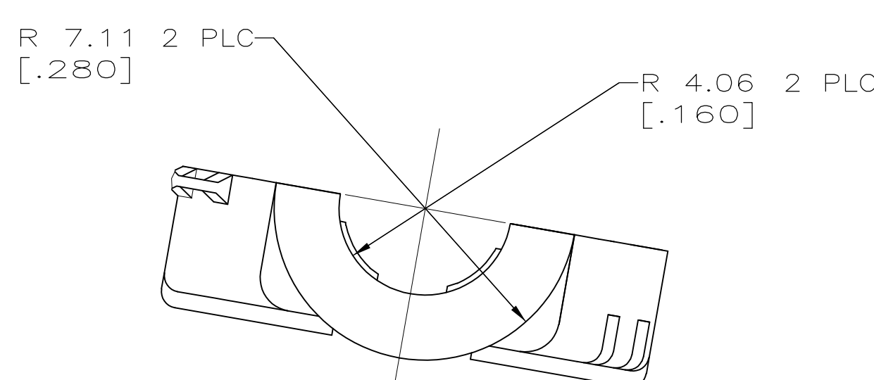
VIEW B-B
