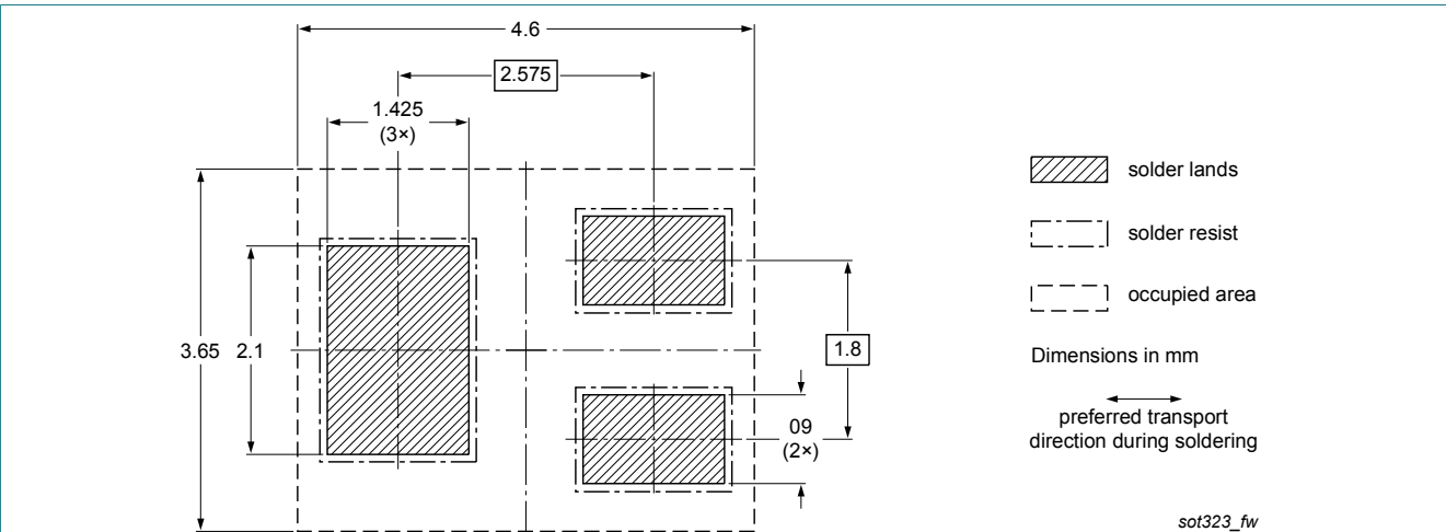
Figure 18. Wave soldering footprint for SOT323 (SC-70)
