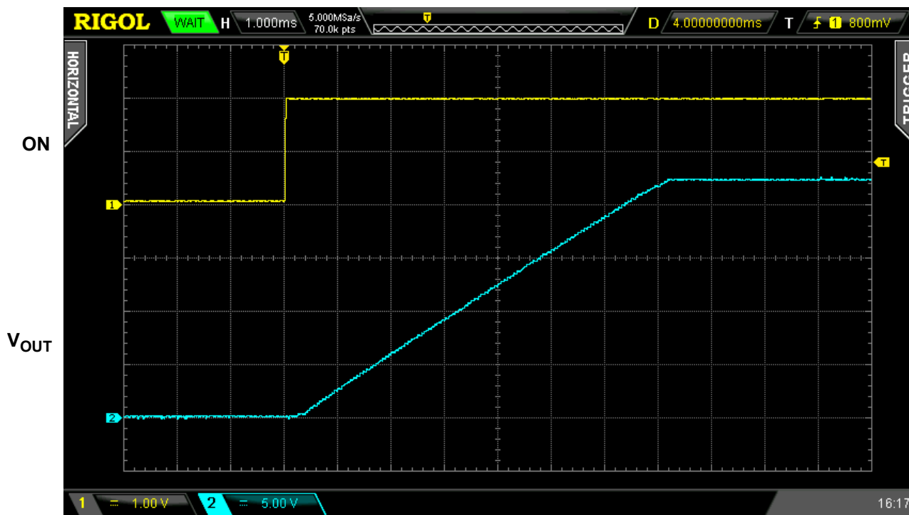
Figure 3. Typical Turn ON operation waveform for V_{IN} = 22\text{ V} , C_{SLEW} = 10\text{ nF} , C_{LOAD} = 10\text{ μF} , R_{LOAD} = 100\text{ Ω}
