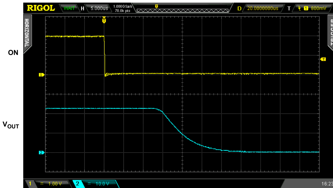
Figure 7. Typical Turn OFF operation waveform for V_{IN} = 22\text{ V} , C_{SLEW} = 10\text{ nF} , no C_{LOAD} , R_{LOAD} = 100\ \Omega
