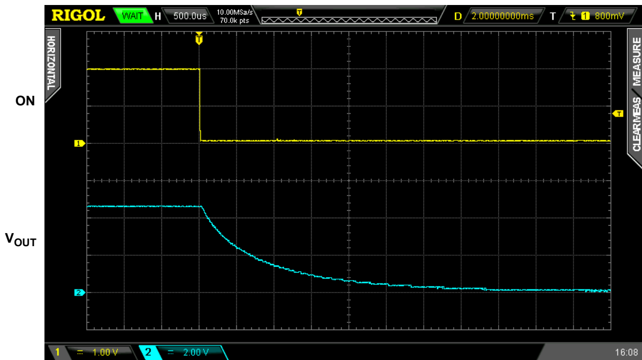
Figure 6. Typical Turn OFF operation waveform for V_{IN} = 4.5\text{ V} , C_{SLEW} = 10\text{ nF} , C_{LOAD} = 10\text{ }\mu\text{F} , R_{LOAD} = 100\text{ }\Omega
