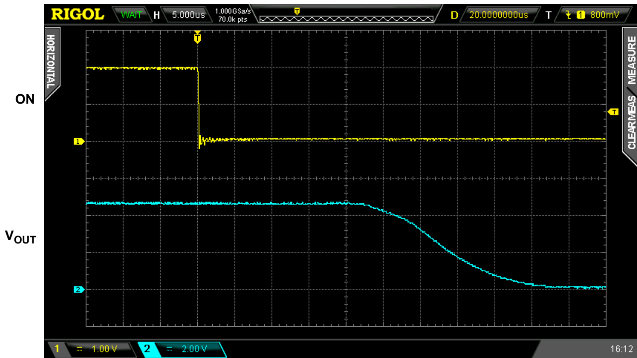
Figure 5. Typical Turn OFF operation waveform for V_{IN} = 4.5\text{ V} , C_{SLEW} = 10\text{ nF} , no C_{LOAD} , R_{LOAD} = 100\text{ }\Omega
