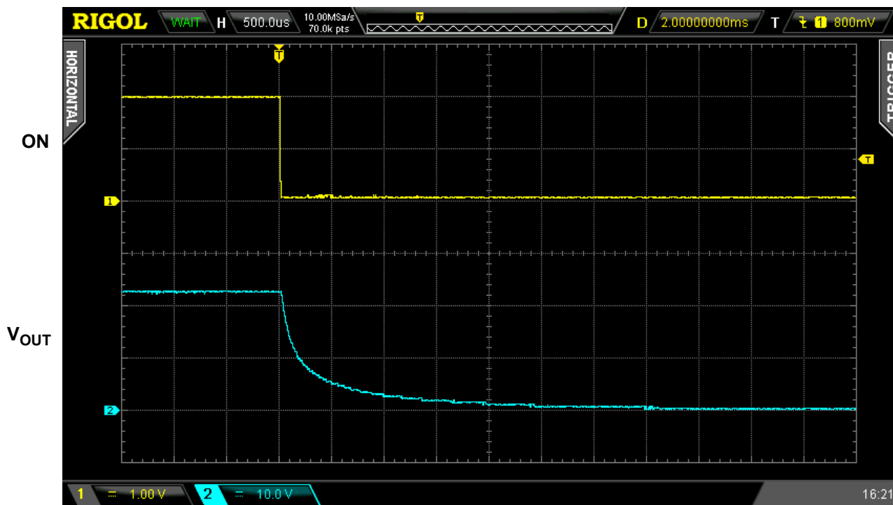
Figure 8. Typical Turn OFF operation waveform for V_{IN} = 22\text{ V} , C_{SLEW} = 10\text{ nF} , C_{LOAD} = 10\ \mu\text{F} , R_{LOAD} = 100\ \Omega
