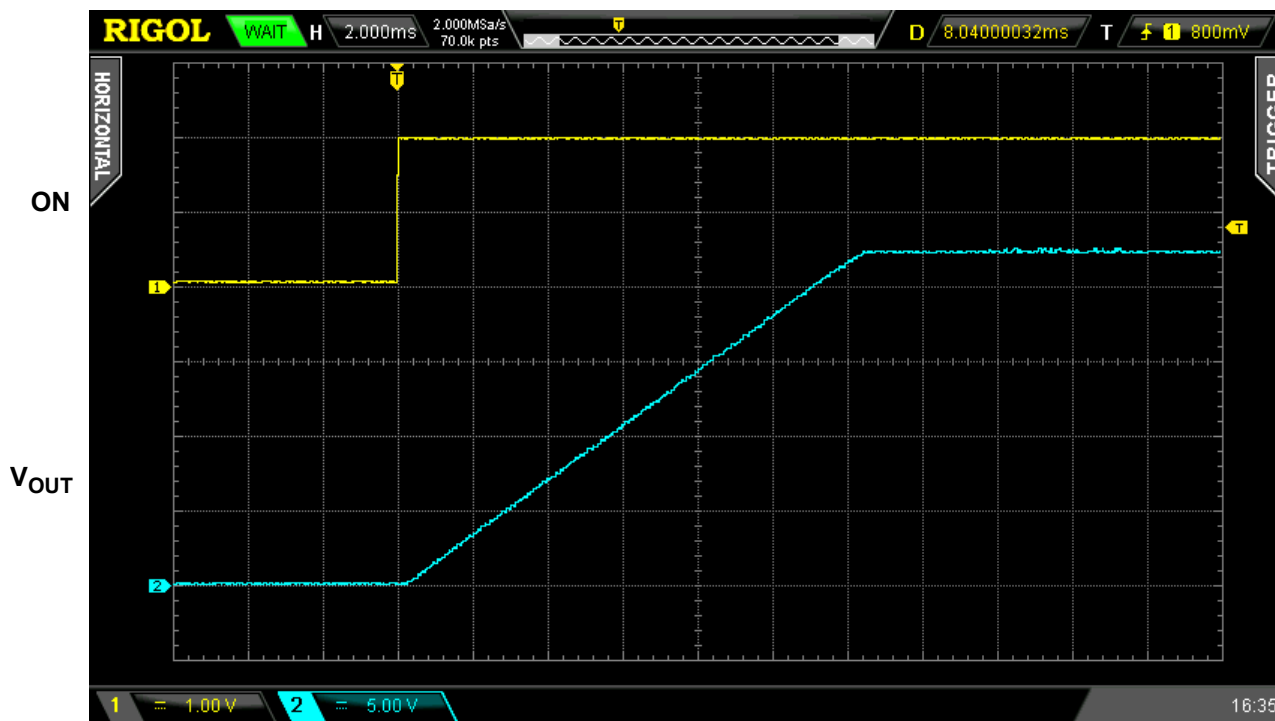
Figure 4. Typical Turn ON operation waveform for V_{IN} = 22\text{ V} , C_{SLEW} = 18\text{ nF} , C_{LOAD} = 10\text{ μF} , R_{LOAD} = 100\text{ Ω}
