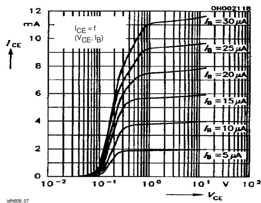
Figure 7. Output Characteristics
