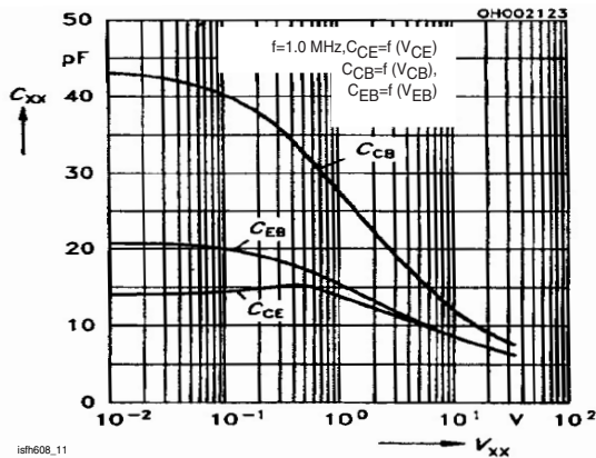
Figure 11. Transistor Capacitance
