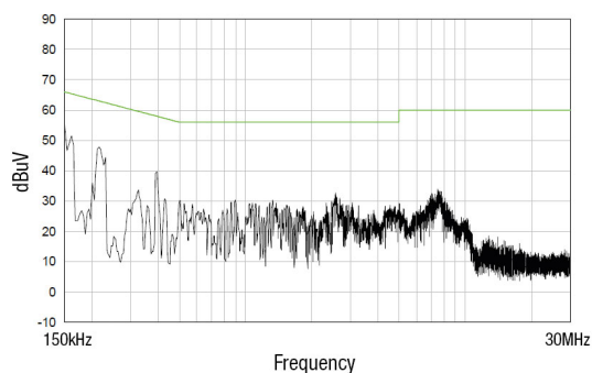
BAC1S24SC (230V) - Live
