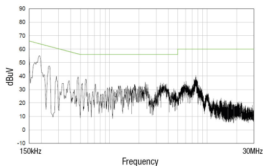
BAC1S12SC (110V) - Neutral
