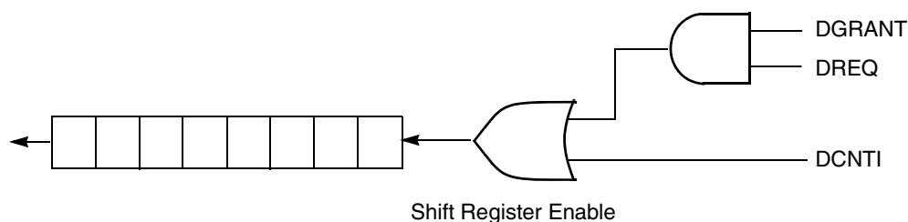
Figure 13-8. D-Channel Contention
