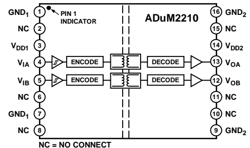
Figure 1. ADuM2210
