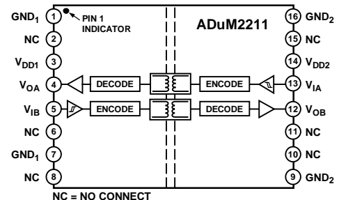
Figure 2. ADuM2211
