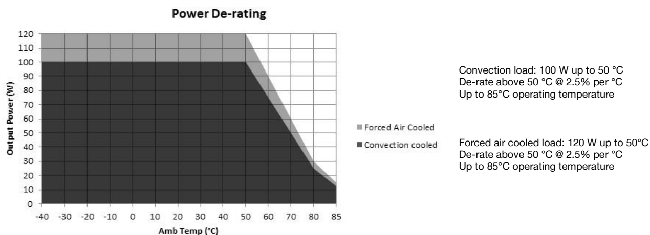
Figure 1. Derating Curve
