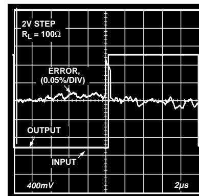
Figure 14. Long-Term Settling Time
