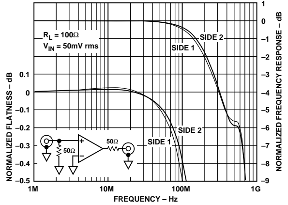
Figure 6. Frequency Response and Flatness
