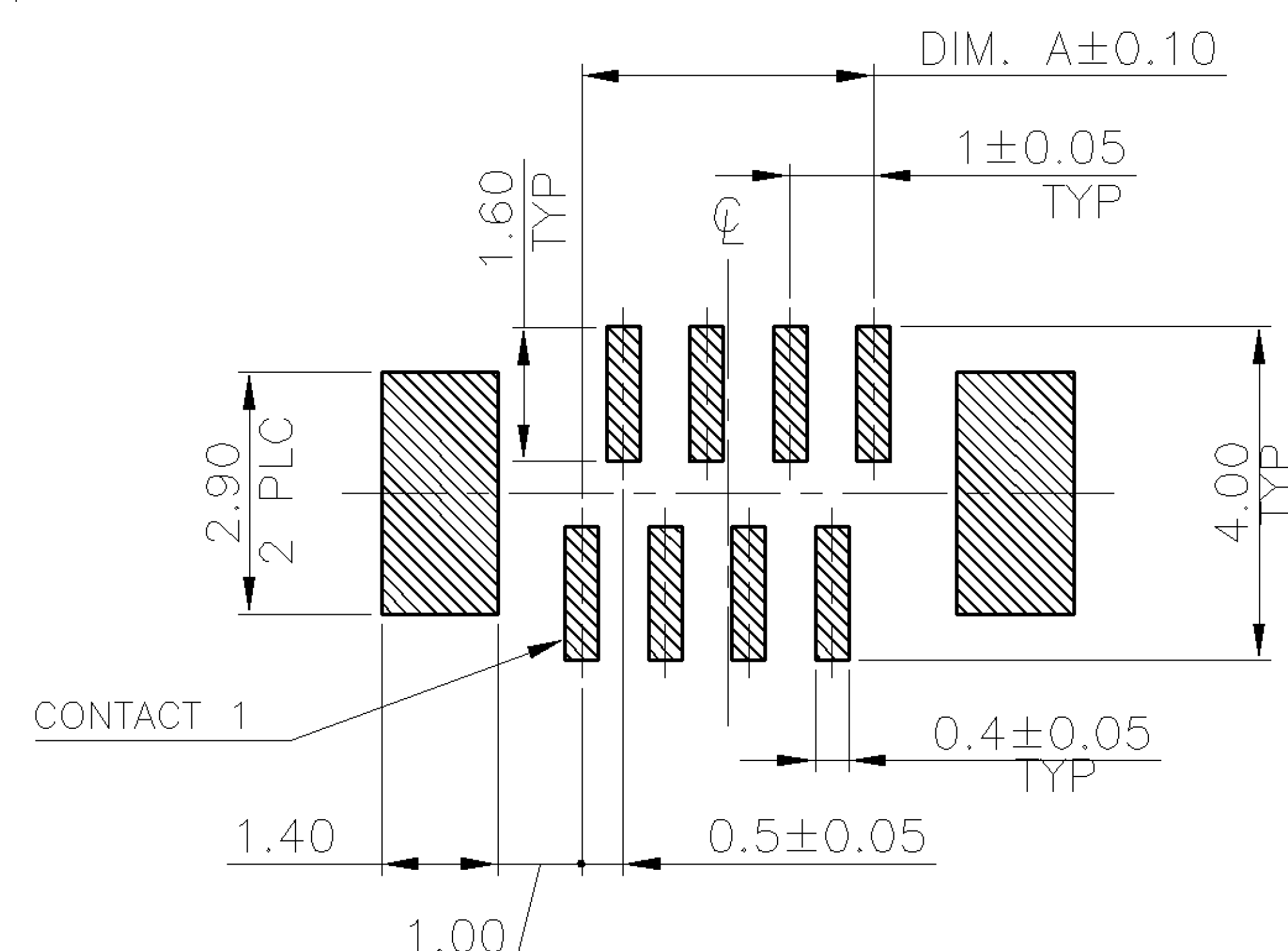
RECOMMENDED PCB LAYOUT (TYPE A) (TOLERANCE: \pm 0.05 )
