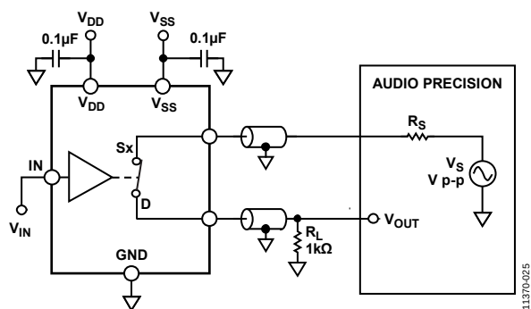
Figure 30. THD + Noise
