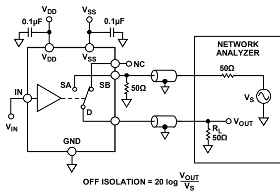
Figure 29. Off Isolation
