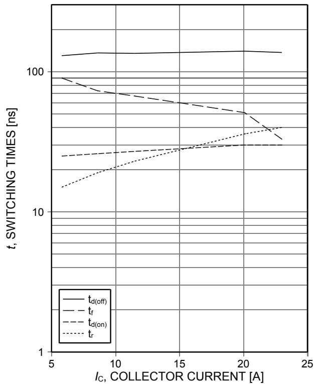
Figure 8. Typical switching times as a function of collector current (inductive load, T_{vj}=150^\circ\text{C} , V_{CE}=400\text{V} , V_{GE}=15/0\text{V} , r_G=47\Omega , Dynamic test circuit in Figure E)
