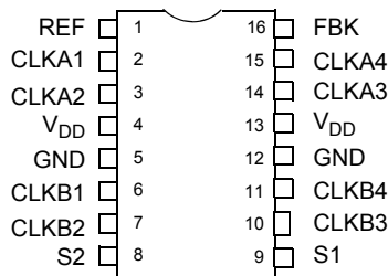
Figure 1. Pin Diagram - 16-pin SOIC (Top View)
