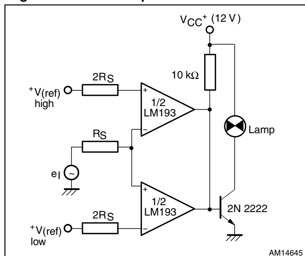
Figure 16. Limit comparator
