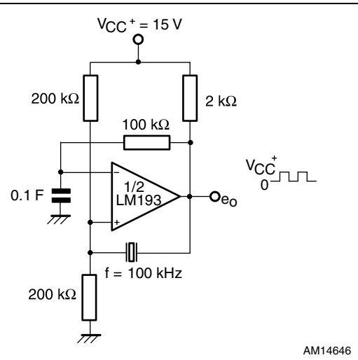
Figure 17. Crystal controlled oscillator
