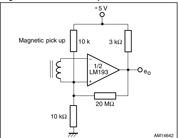
Figure 13. Transducer amplifier
