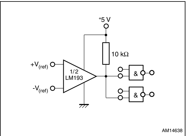
Figure 11. Driving CMOS
