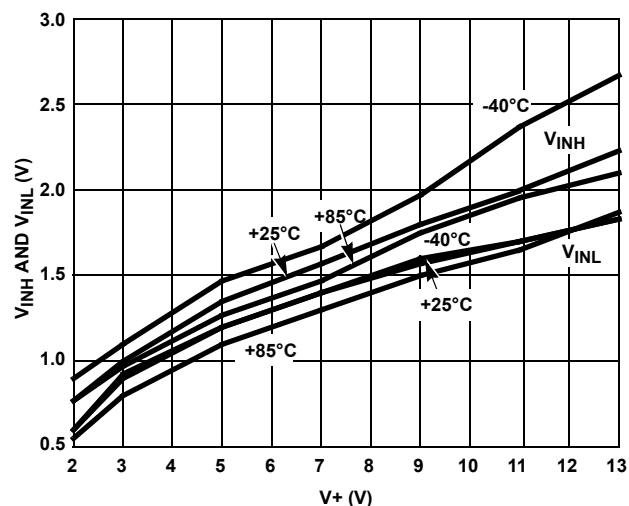
FIGURE 10. DIGITAL SWITCHING POINT vs SUPPLY VOLTAGE
