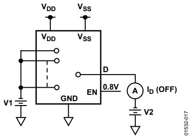
Figure 17. I_D (Off)
