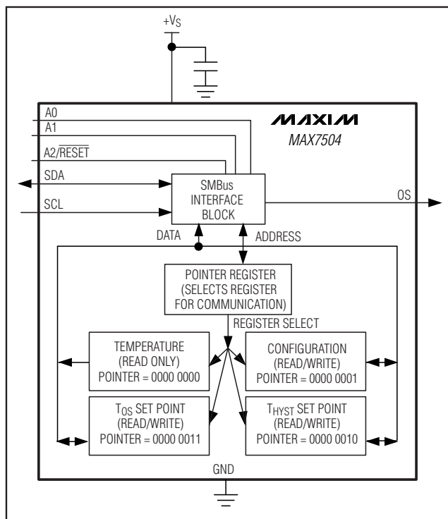
Figure 5. Block Diagram
