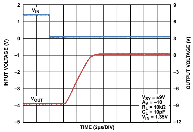
Figure 53. Negative Overload Recovery
