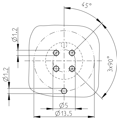
PCB-layout (advice)
