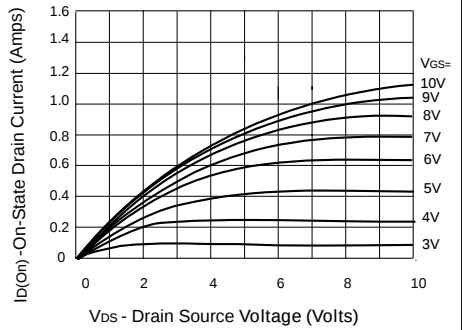
Saturation Characteristics
