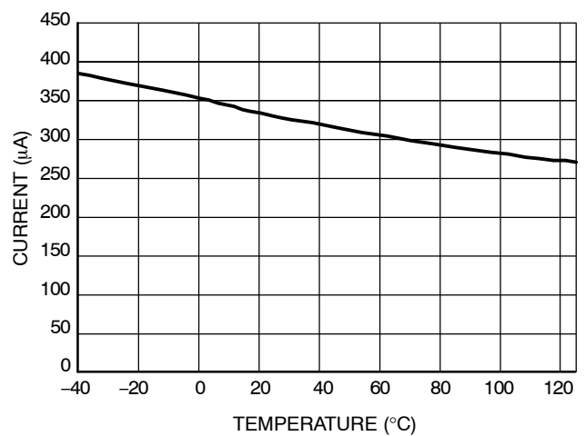
Figure 15. I_{CC4}
