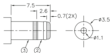
MATING PLUG
