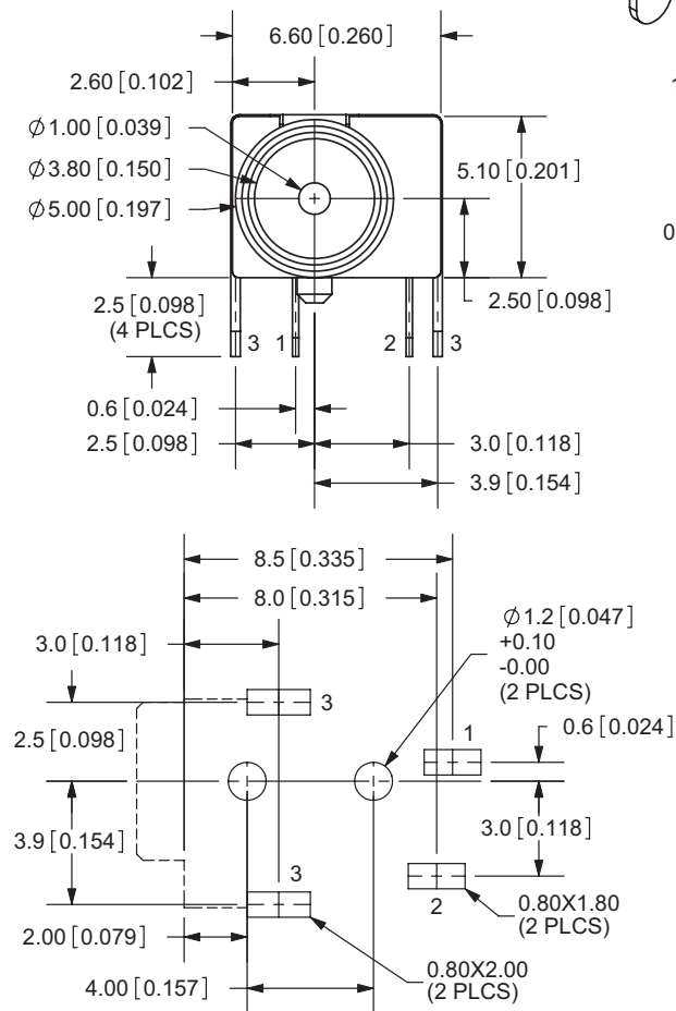
PCB LAYOUT TOP VIEW
