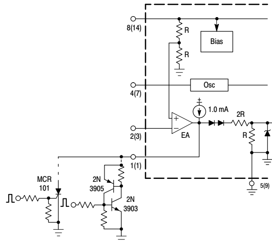
Figure 31. Latched Shutdown
