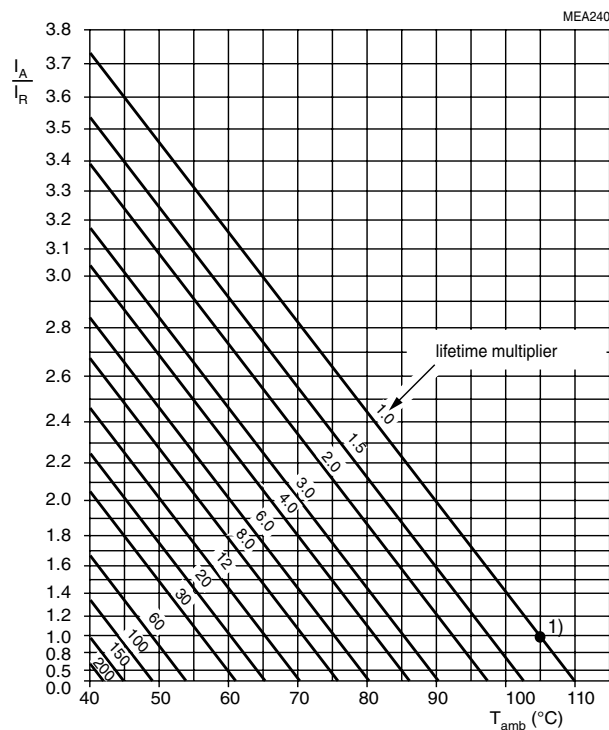
Fig.13 Multiplier of useful life as a function of ambient temperature and ripple current load
