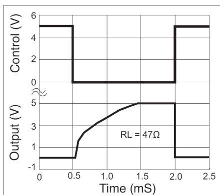
Fig. 12: Turn-on/Turn-off Characteristics
