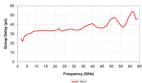
Group Delay
