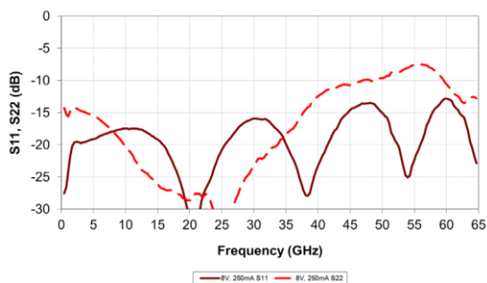
S11, S22
