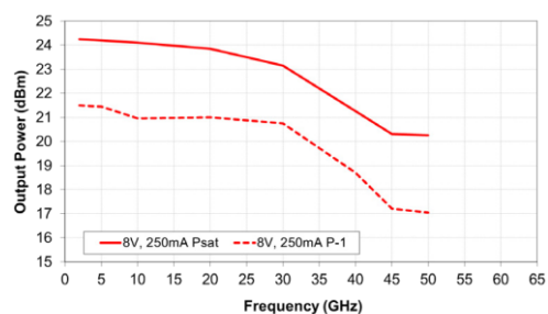
Output Power
