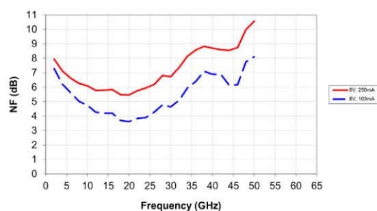
Noise Frequency
