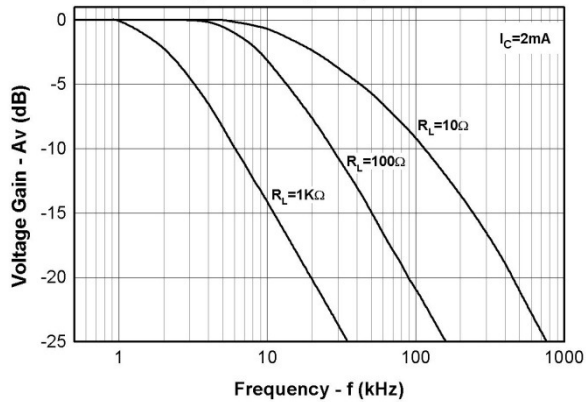
Figure 9. Frequency Response
