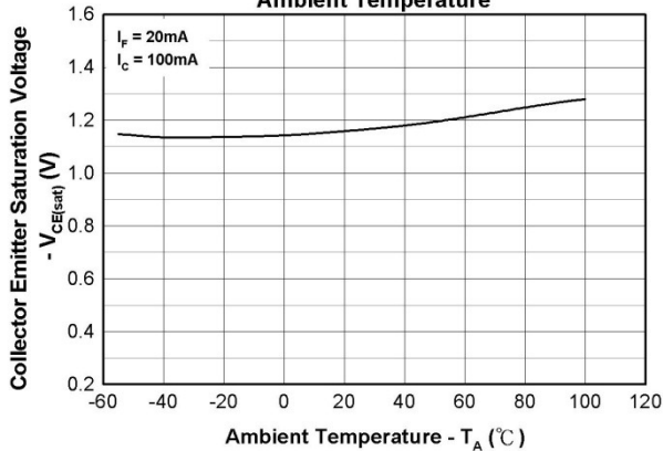
Figure 3. Collector Emitter Saturation Voltage vs. Ambient Temperature
