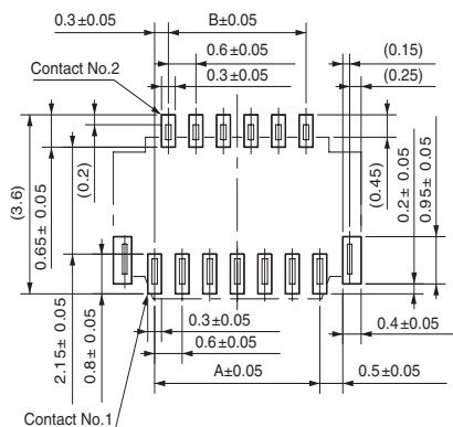
Recommended FPC Dimensions
