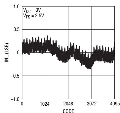
Integral Nonlinearity (LTC2631A-LM12)
