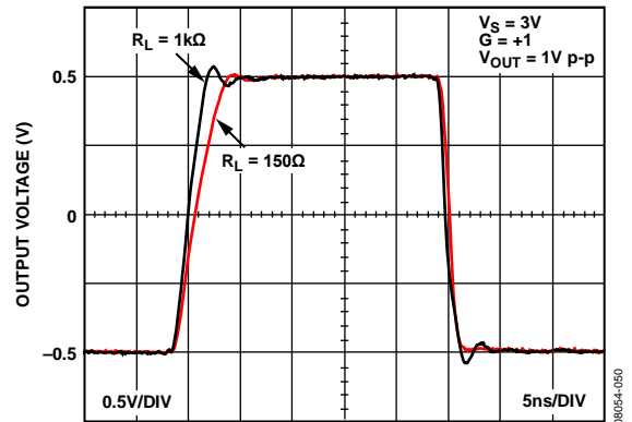
Figure 36. Large-Signal Step Response, V_S = 3\text{ V} , G = +1
