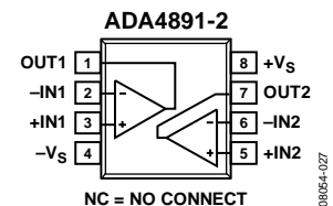
Figure 3. 8-Lead SOIC N (R-8) and 8-Lead MSOP (RM-8)
