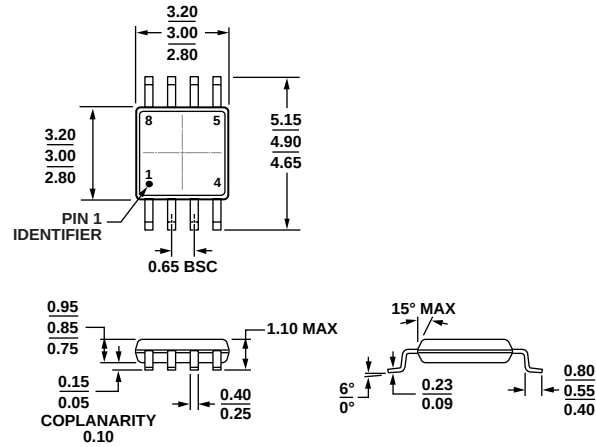
Figure 70. 8-Lead Mini Small Outline Package [MSOP] (RM-8) Dimensions shown in millimeters
