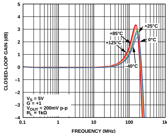
Figure 9. Small-Signal Frequency Response vs. Temperature, V_S = 5\text{ V} , ADA4891-1/ADA4891-2
