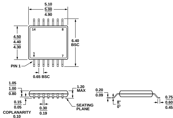
Figure 71. 14-Lead Standard Small Outline Package [SOIC_N] Narrow Body (R-14) Dimensions shown in millimeters and (inches)
