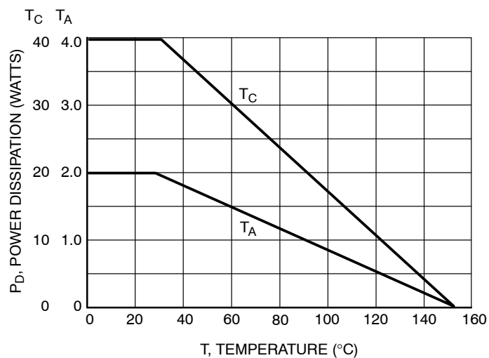
Figure 2. Power Derating
