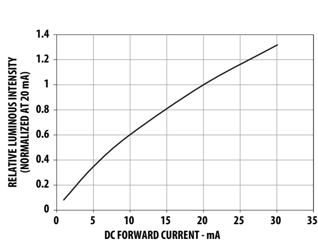
Figure 4: Relative Intensity vs. Forward Current
