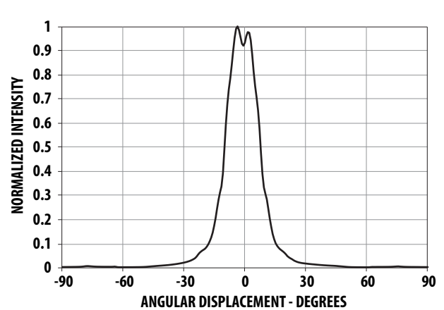
Figure 7: Representative Radiation Pattern for 15° Viewing Angle Lamp
