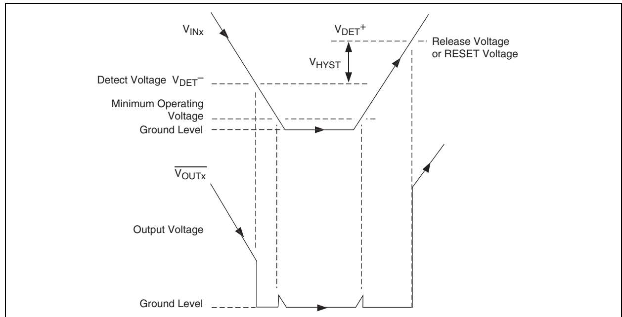
FIGURE 3-1: TIMING DIAGRAM
