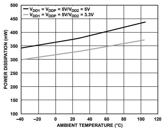
Figure 16. Power Dissipation with a 30 mA Load vs. Temperature
