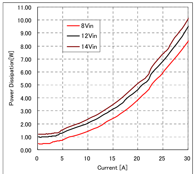
Fig-5.0V-3: Power Loss vs. load current and input voltage for V_{out}=5.0V . Airflow rate=200 LFM (1m/s) and T_a=25^{\circ}C .
