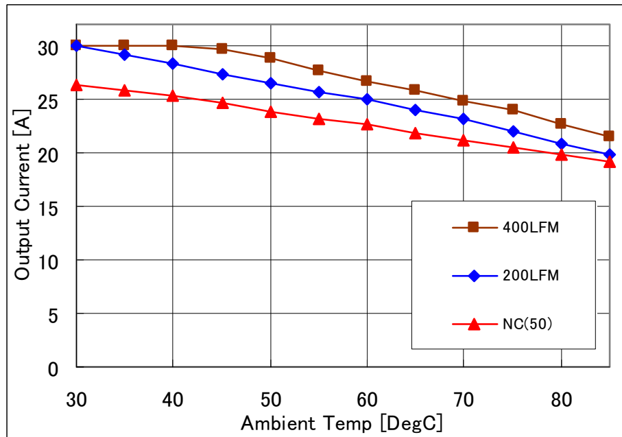
Fig-5.0V-1: Available load current vs. ambient temperature and airflow rates for V_{out}=5.0V with V_{in}=12V . Maximum component temperature \leq 120^{\circ}C
