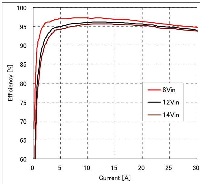
Fig-5.0V-2: Efficiency vs. load current and input voltage for V_{out}=5.0V . Airflow rate=200 LFM (1m/s) and T_a=25^{\circ}C .
