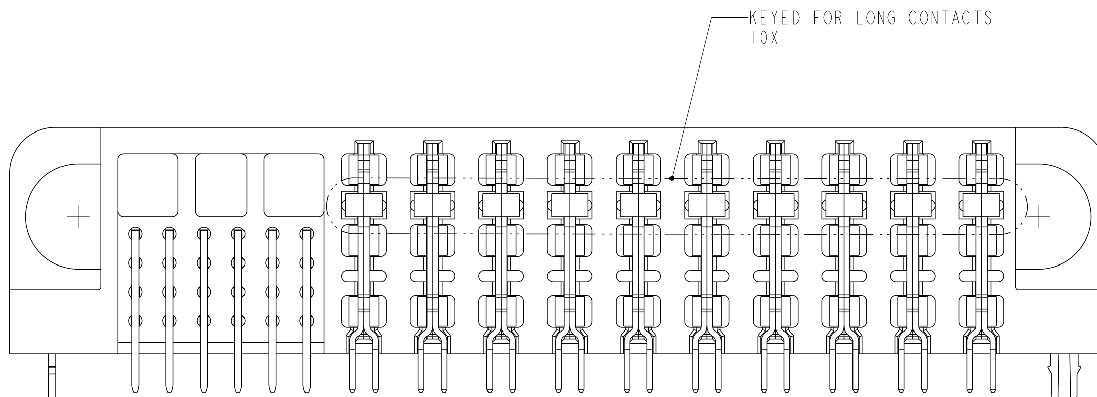
VIEW G-G
