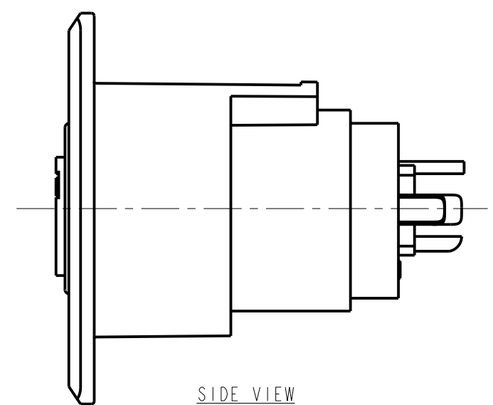
FIGURE 1 3 PIN DETENT VERSION (NO LATCH)
