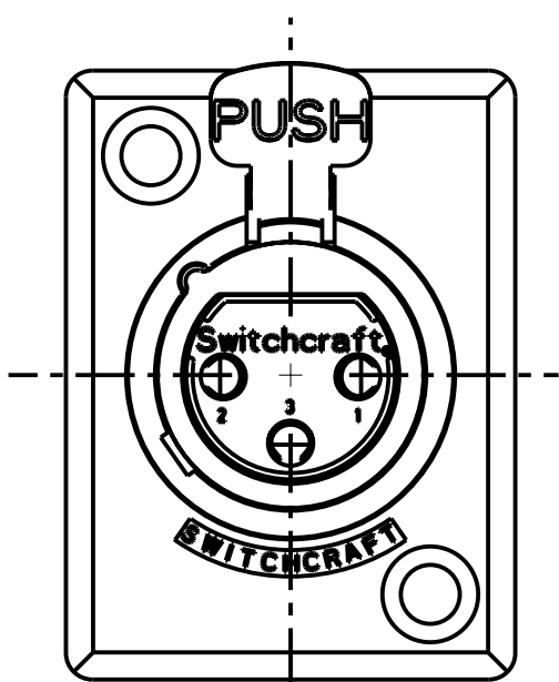
3 PIN
