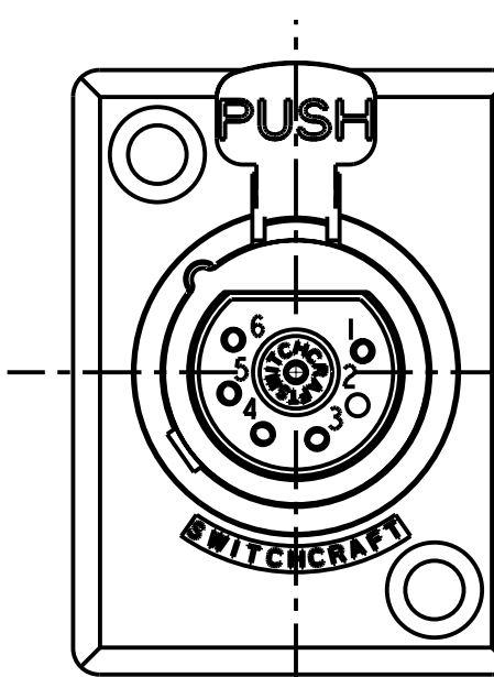
7 PIN
