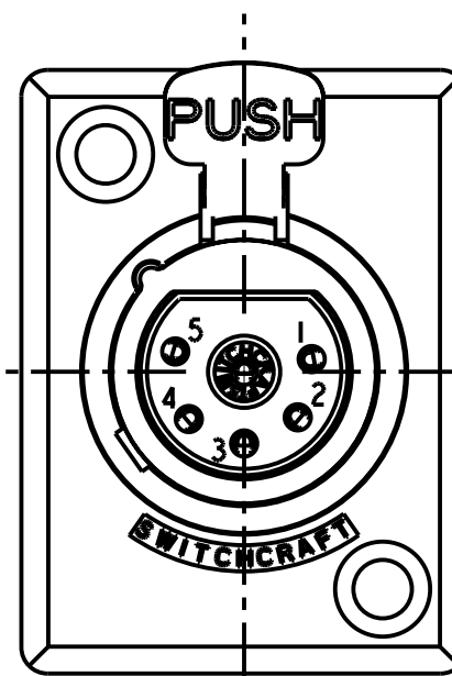
6 PIN
