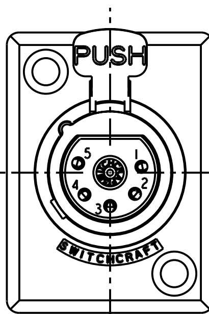
5 PIN
