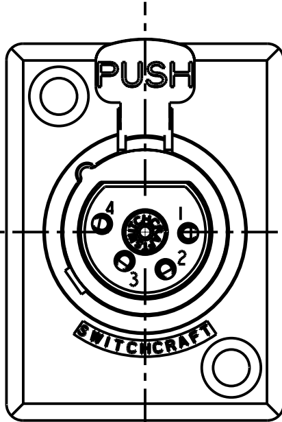
4 PIN
