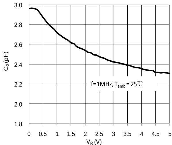
Figure 4. Input Capacitance vs. Input Voltage
