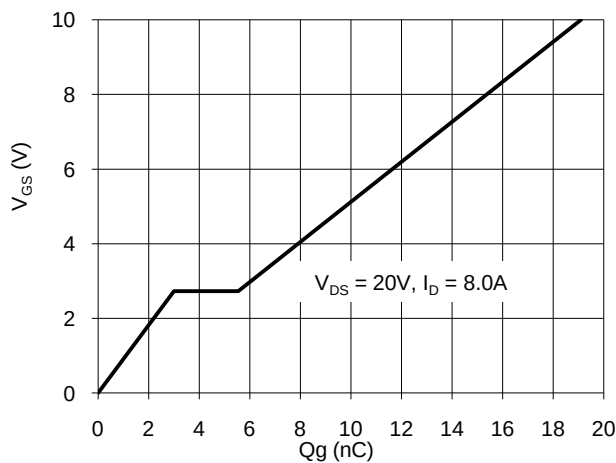
Figure 11. Gate Charge
