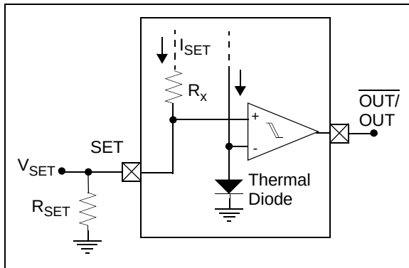
FIGURE 4-1: SET input.
